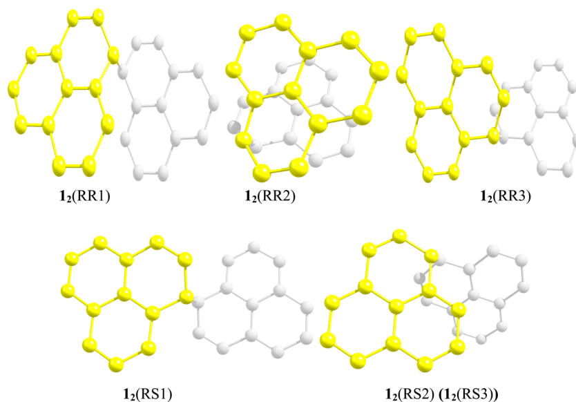
Figure 3. Optimized geometries of I_2 \sigma -dimers. Hydrogen atoms are omitted for clarity.
